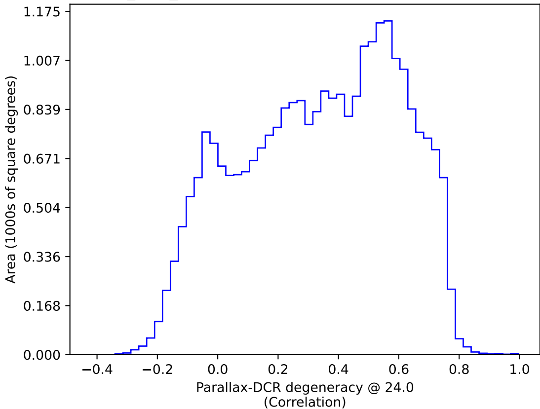
baseline_v3.3_10yrs All sky: Parallax-DCR degeneracy @ 24.0
