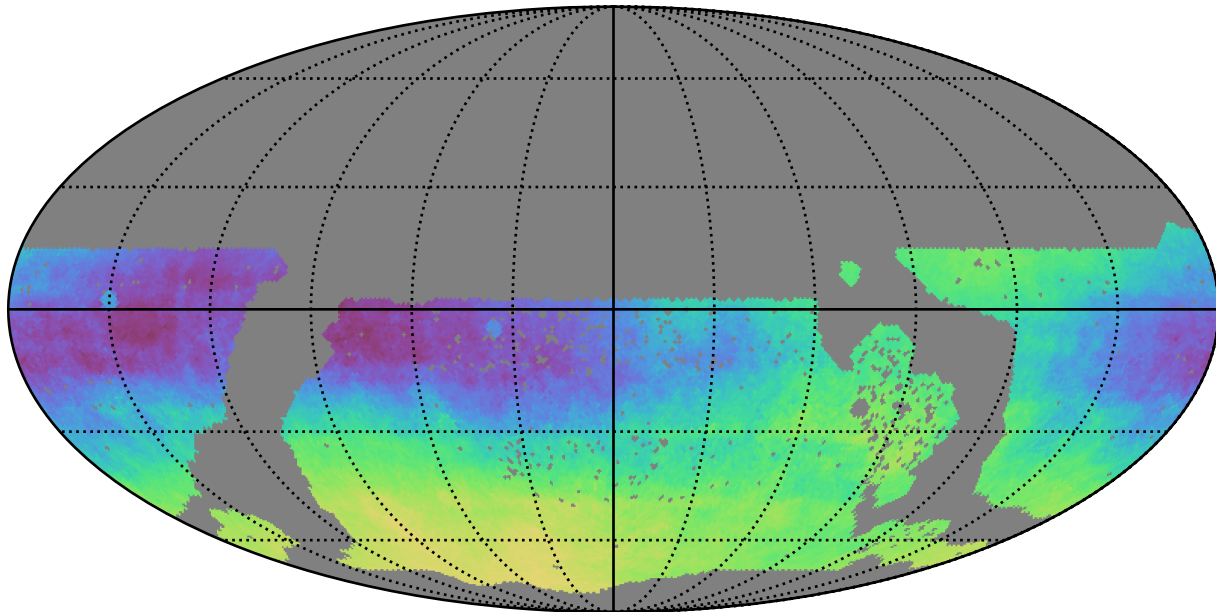
baseline_v3.3_10yrs WFD: Parallax-DCR degeneracy @ 22.4
