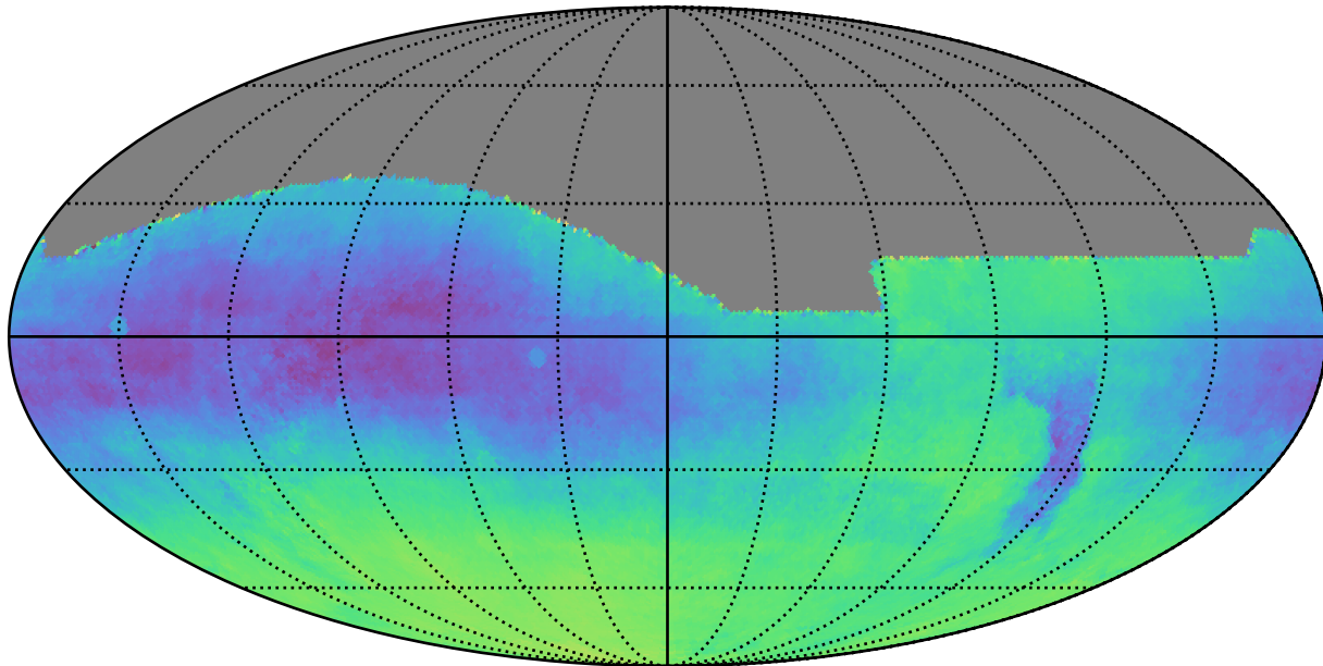
baseline_v3.3_10yrs All sky: Parallax-DCR degeneracy @ 22.4
