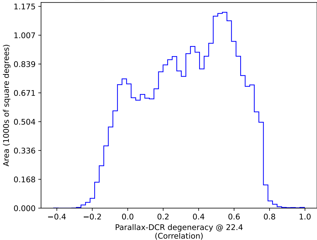
baseline_v3.3_10yrs All sky: Parallax-DCR degeneracy @ 22.4
