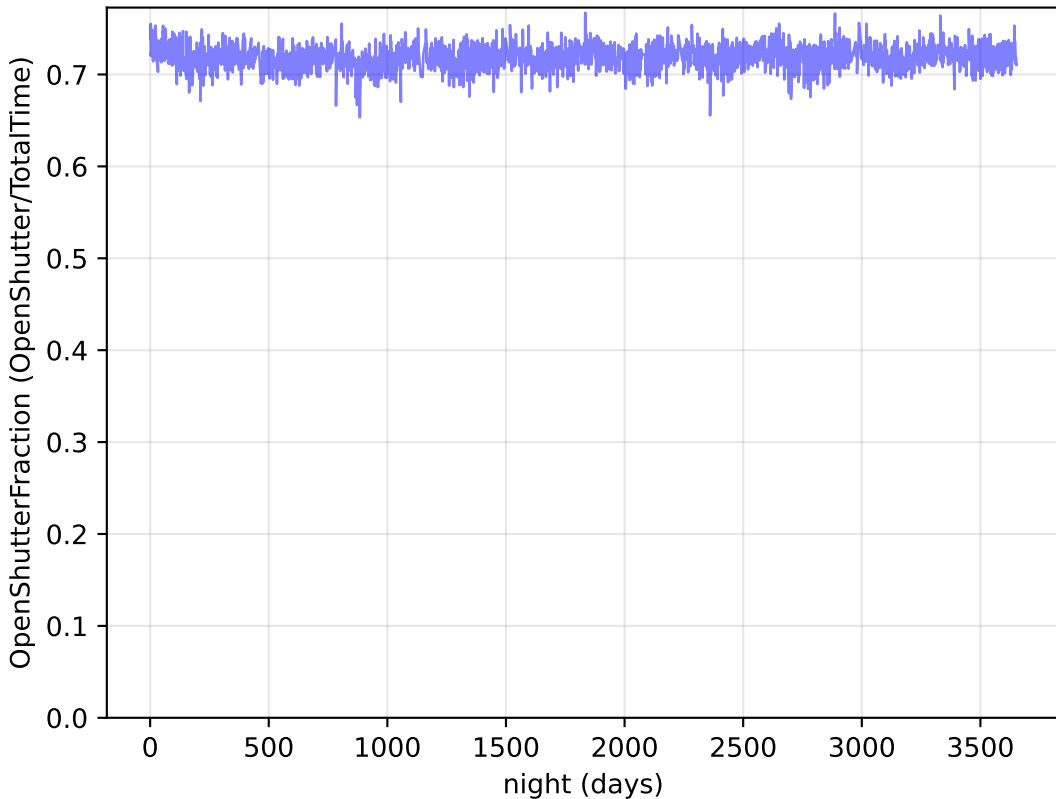
baseline_v3.3_10yrs Per night: OpenShutterFraction
