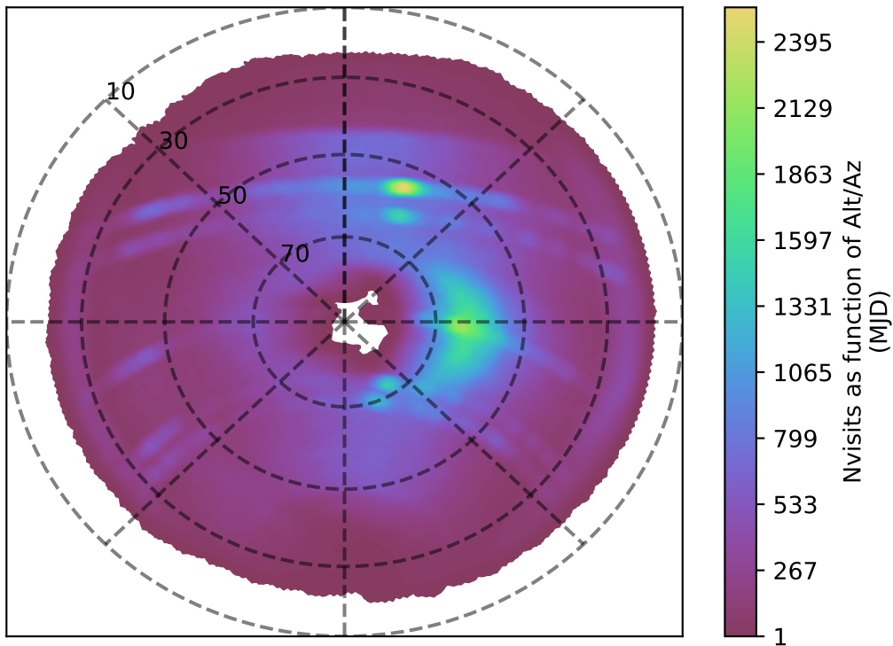
baseline_v3.3_10yrs z band: Nvisits as function of Alt/Az
