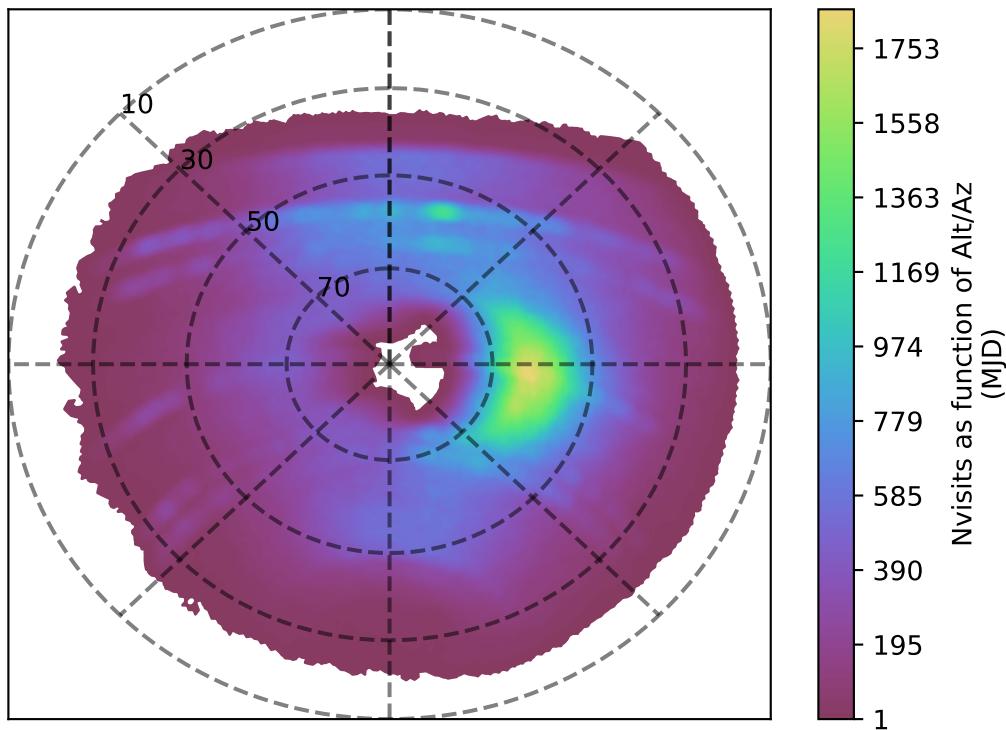
baseline_v3.3_10yrs y band: Nvisits as function of Alt/Az
