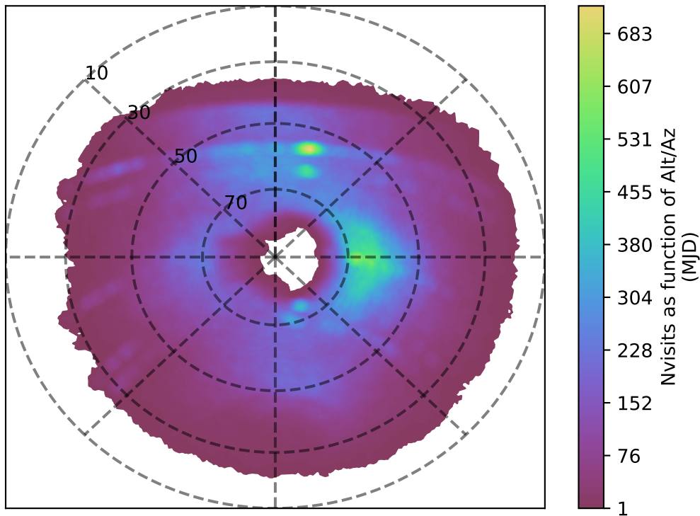
baseline_v3.3_10yrs u band: Nvisits as function of Alt/Az
