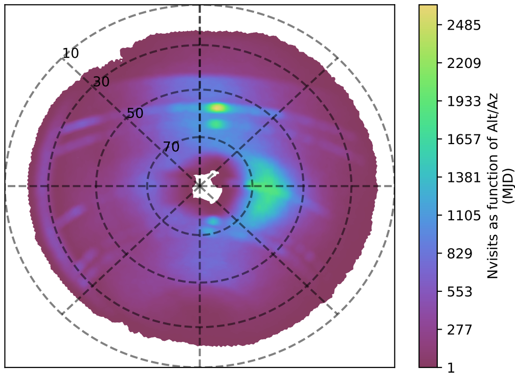
baseline_v3.3_10yrs r band: Nvisits as function of Alt/Az
