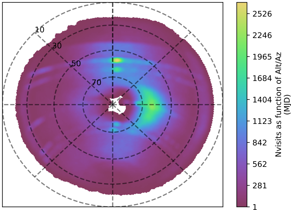
baseline_v3.3_10yrs i band: Nvisits as function of Alt/Az
