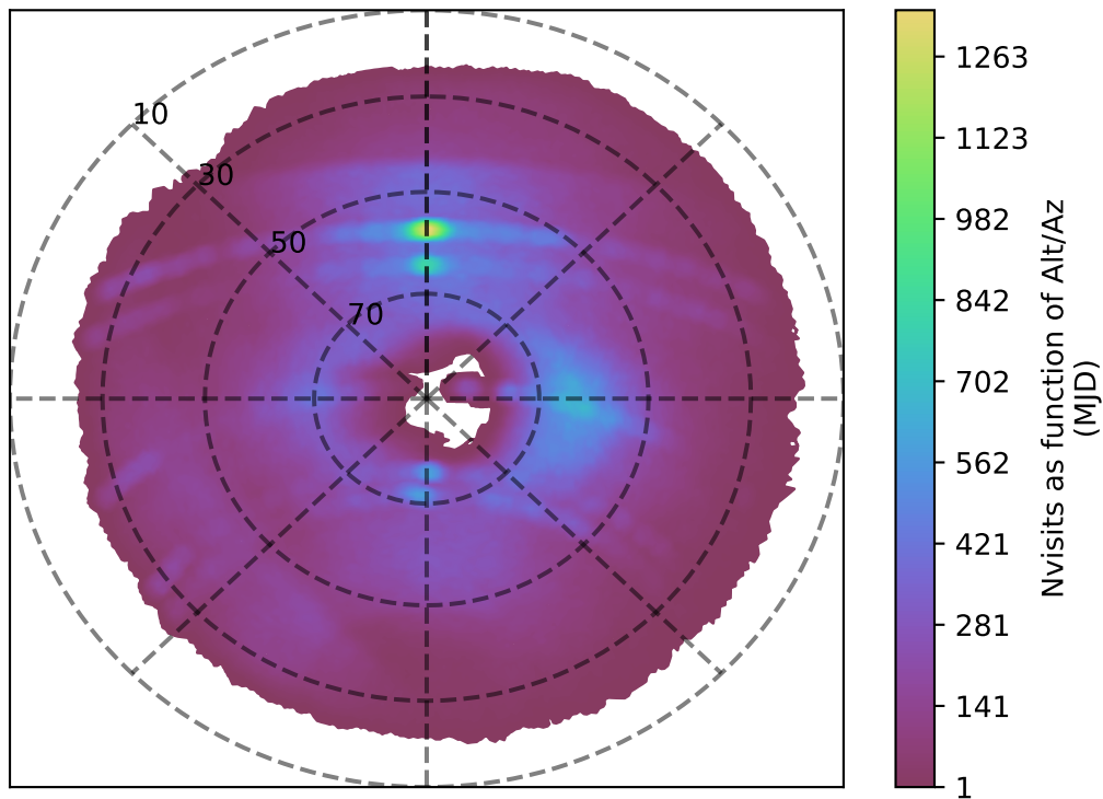
baseline_v3.3_10yrs g band: Nvisits as function of Alt/Az
