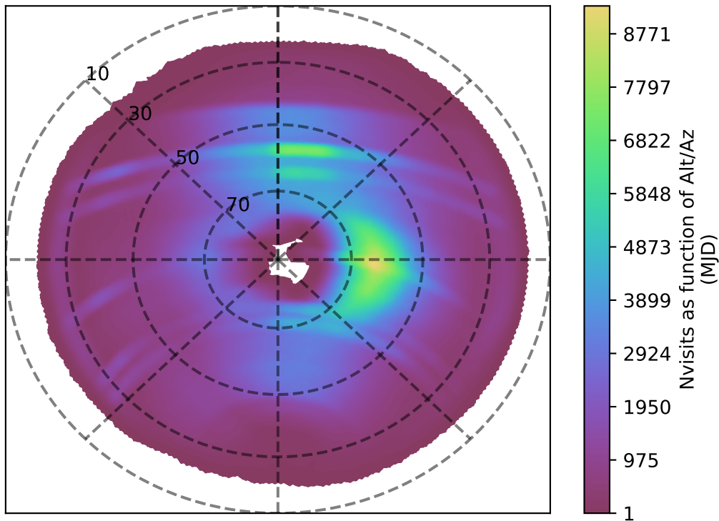
baseline_v3.3_10yrs all bands: Nvisits as function of Alt/Az
