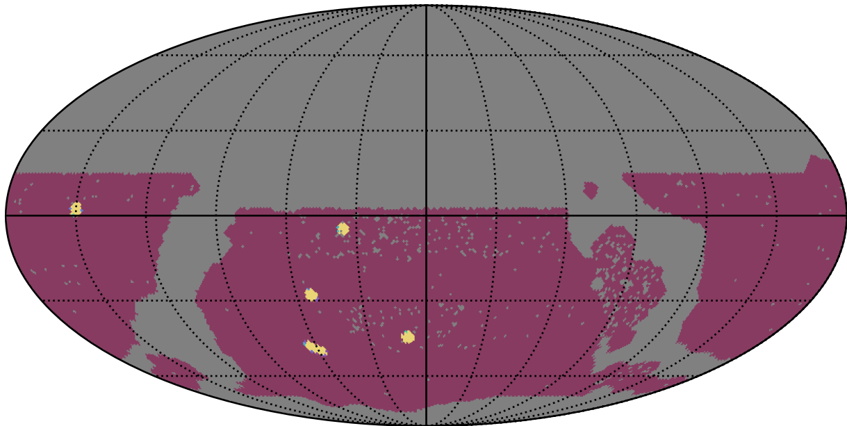
baseline_v3.3_10yrs WFD: NumberOfQuickRevisits
