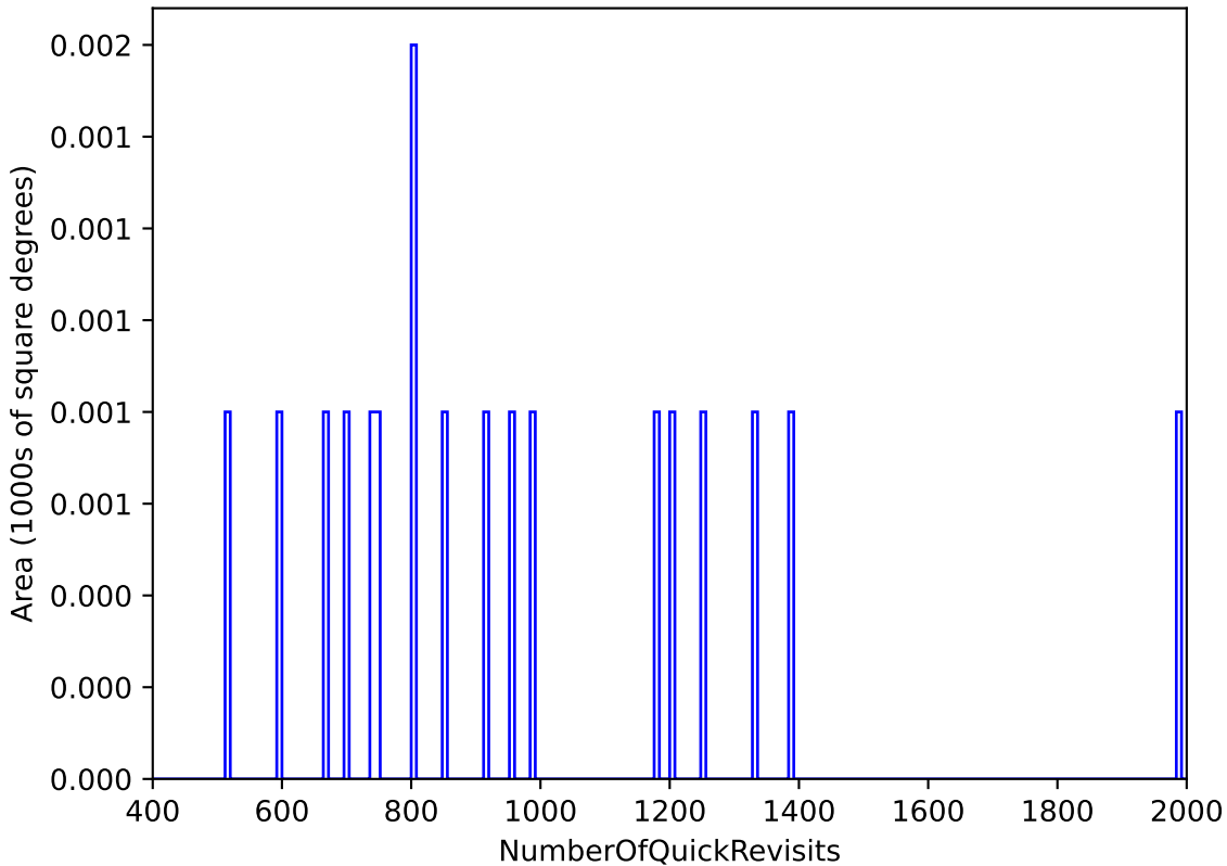
baseline_v3.3_10yrs WFD: NumberOfQuickRevisits
