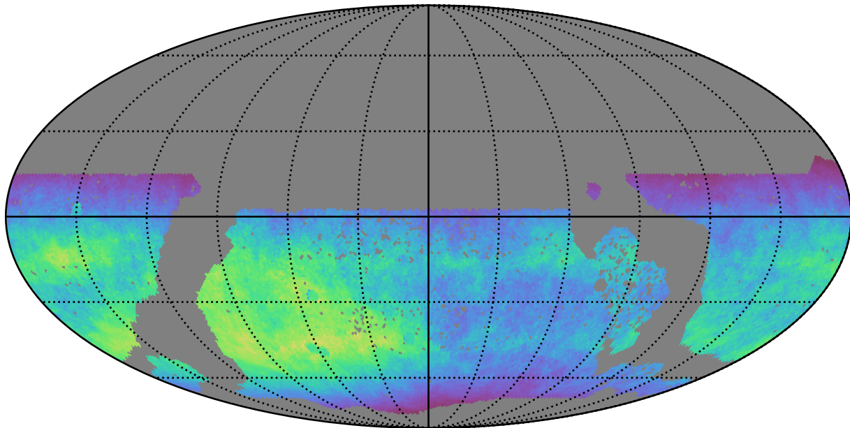
baseline_v3.3_10yrs WFD z band: Normalized Teff
