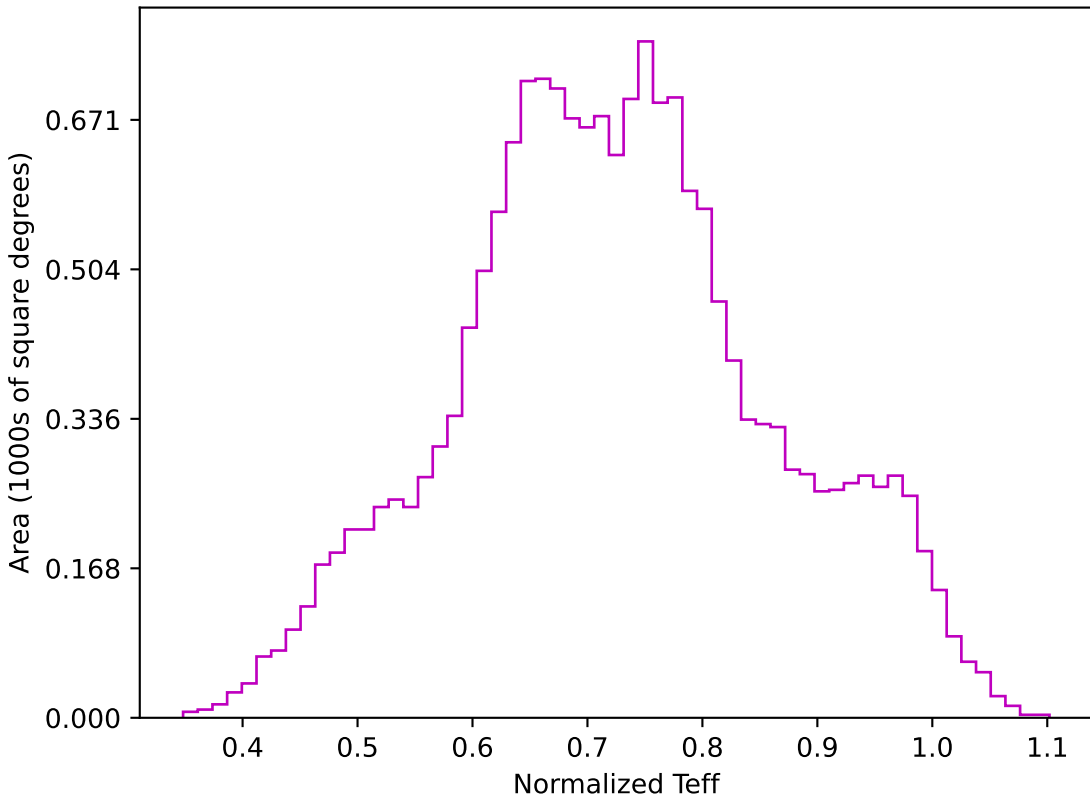
baseline_v3.3_10yrs WFD z band: Normalized Teff
