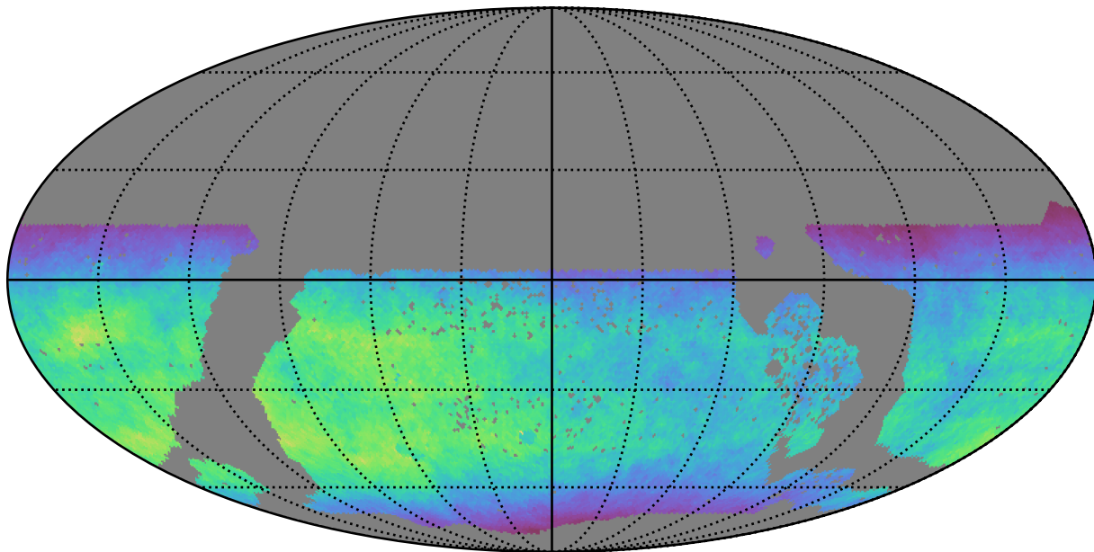
baseline_v3.3_10yrs WFD y band: Normalized Teff
