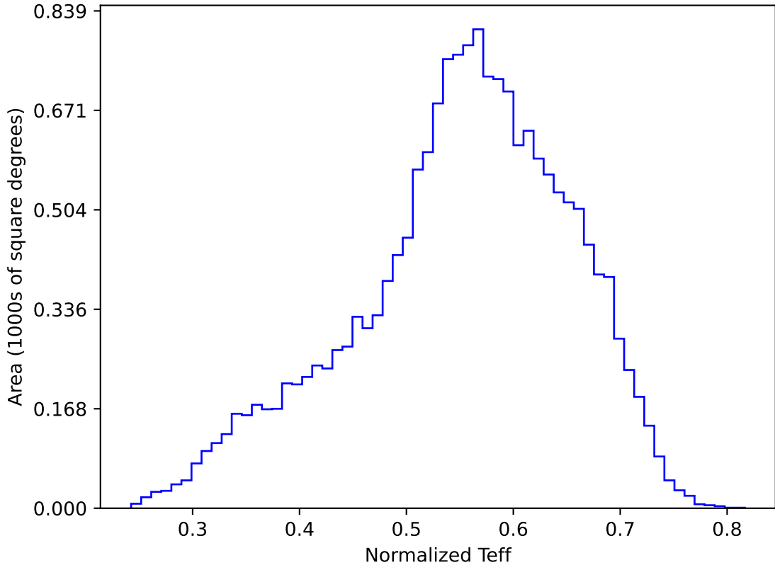
baseline_v3.3_10yrs WFD y band: Normalized Teff
