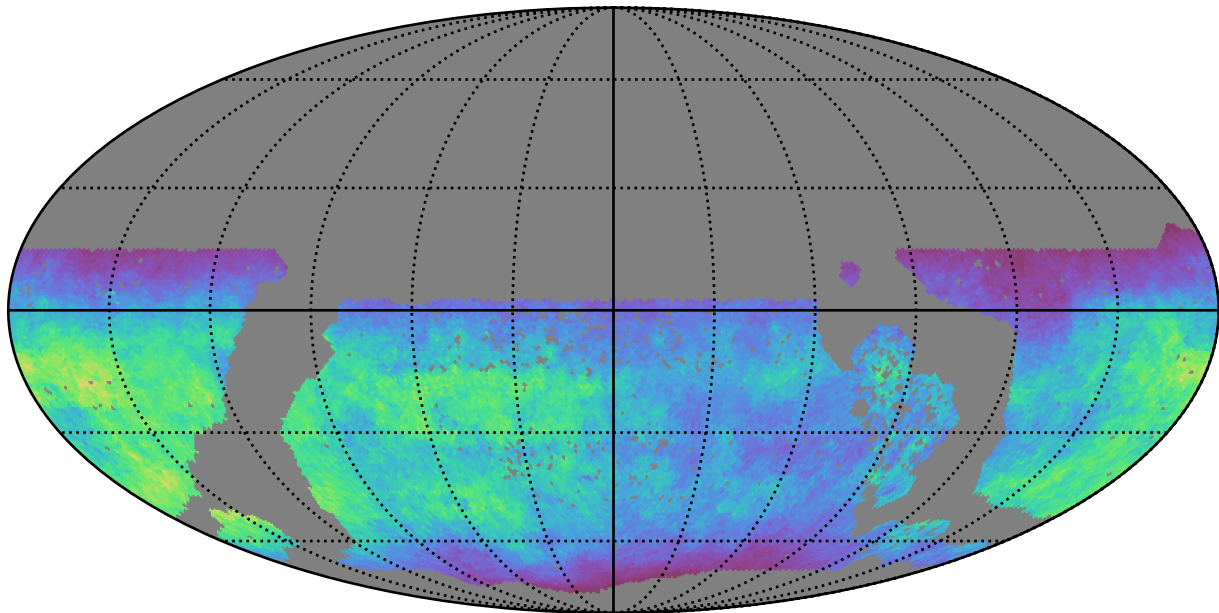
baseline_v3.3_10yrs WFD u band: Normalized Teff
