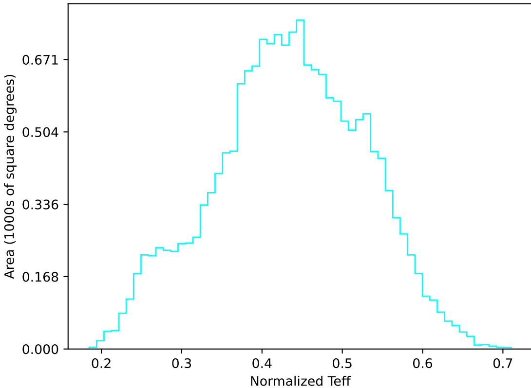
baseline_v3.3_10yrs WFD u band: Normalized Teff
