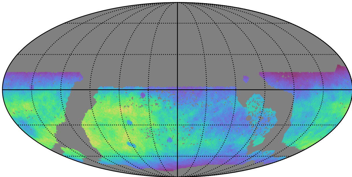
baseline_v3.3_10yrs WFD r band: Normalized Teff
