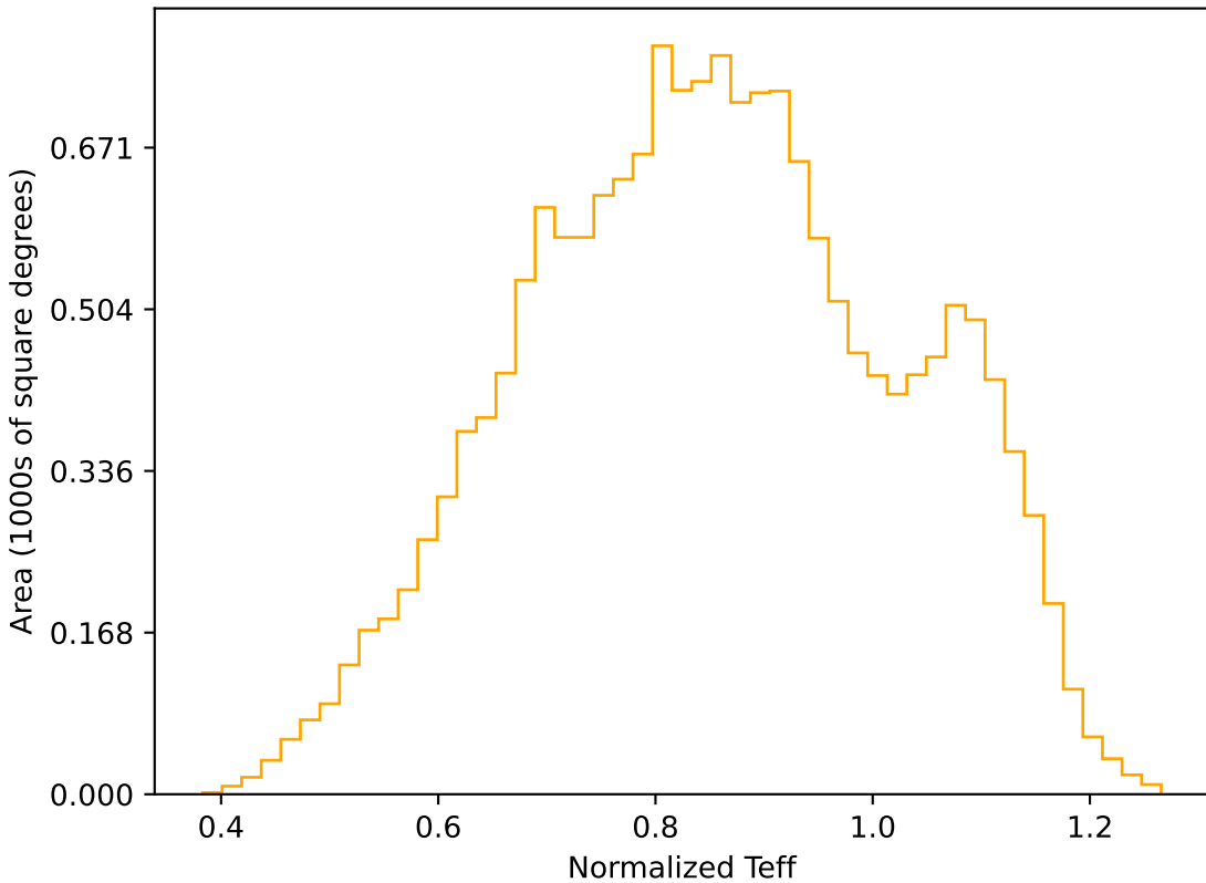
baseline_v3.3_10yrs WFD r band: Normalized Teff
