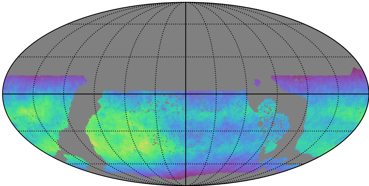
baseline_v3.3_10yrs WFD i band: Normalized Teff
