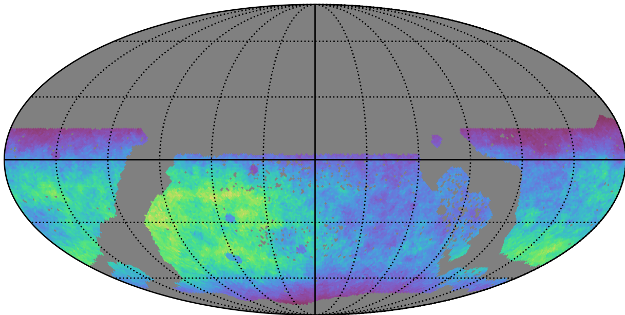
baseline_v3.3_10yrs WFD g band: Normalized Teff
