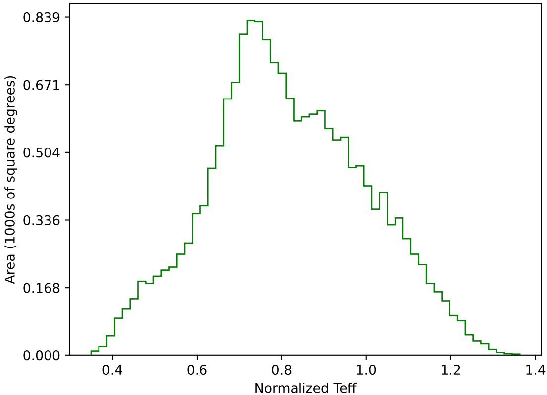
baseline_v3.3_10yrs WFD g band: Normalized Teff
