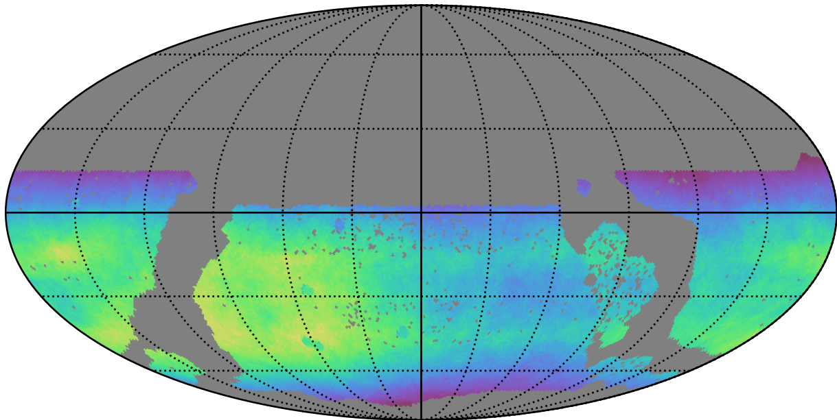
baseline_v3.3_10yrs WFD all bands: Normalized Teff
