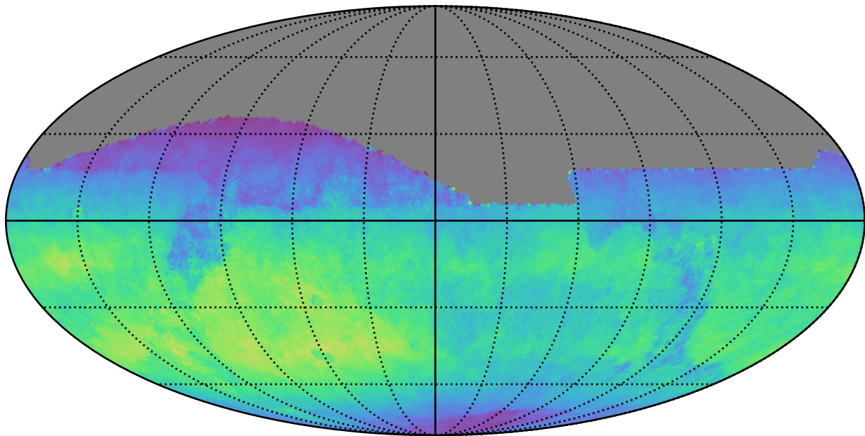
baseline_v3.3_10yrs All sky z band: Normalized Teff
