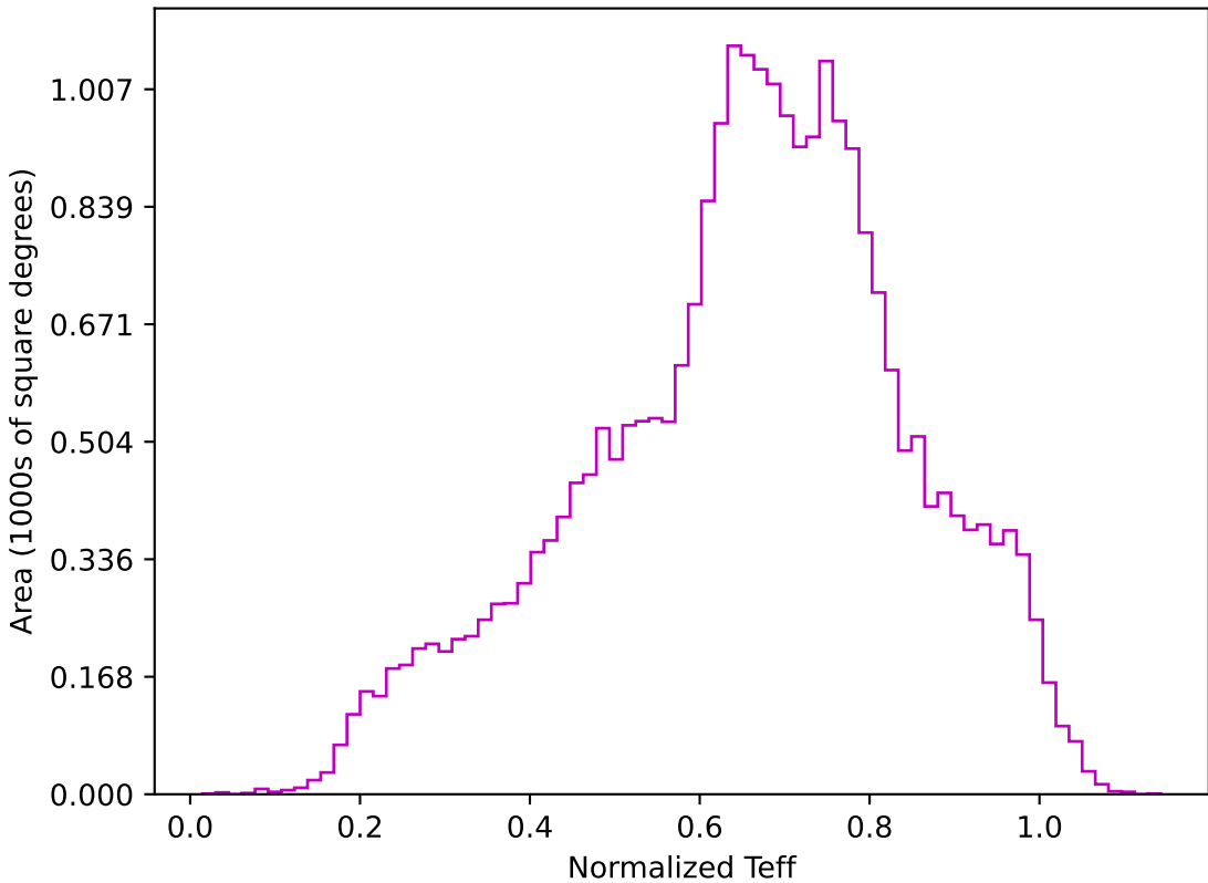
baseline_v3.3_10yrs All sky z band: Normalized Teff
