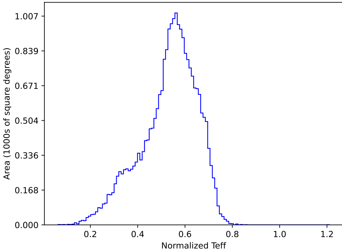
baseline_v3.3_10yrs All sky y band: Normalized Teff
