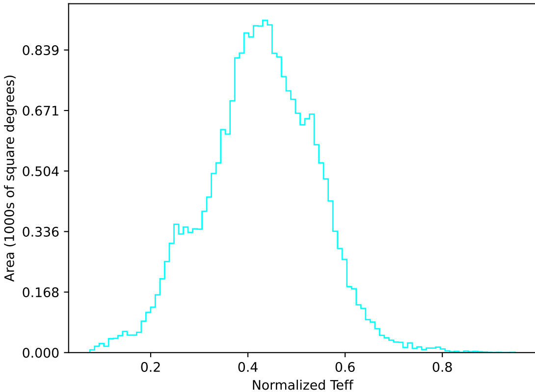
baseline_v3.3_10yrs All sky u band: Normalized Teff
