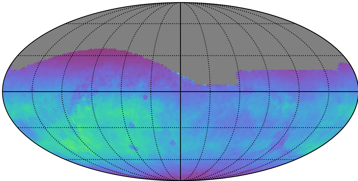
baseline_v3.3_10yrs All sky r band: Normalized Teff
