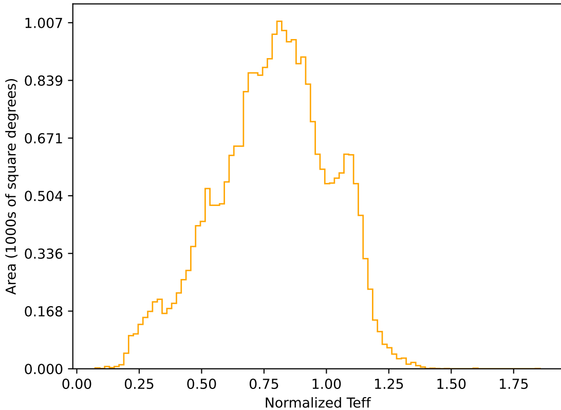
baseline_v3.3_10yrs All sky r band: Normalized Teff
