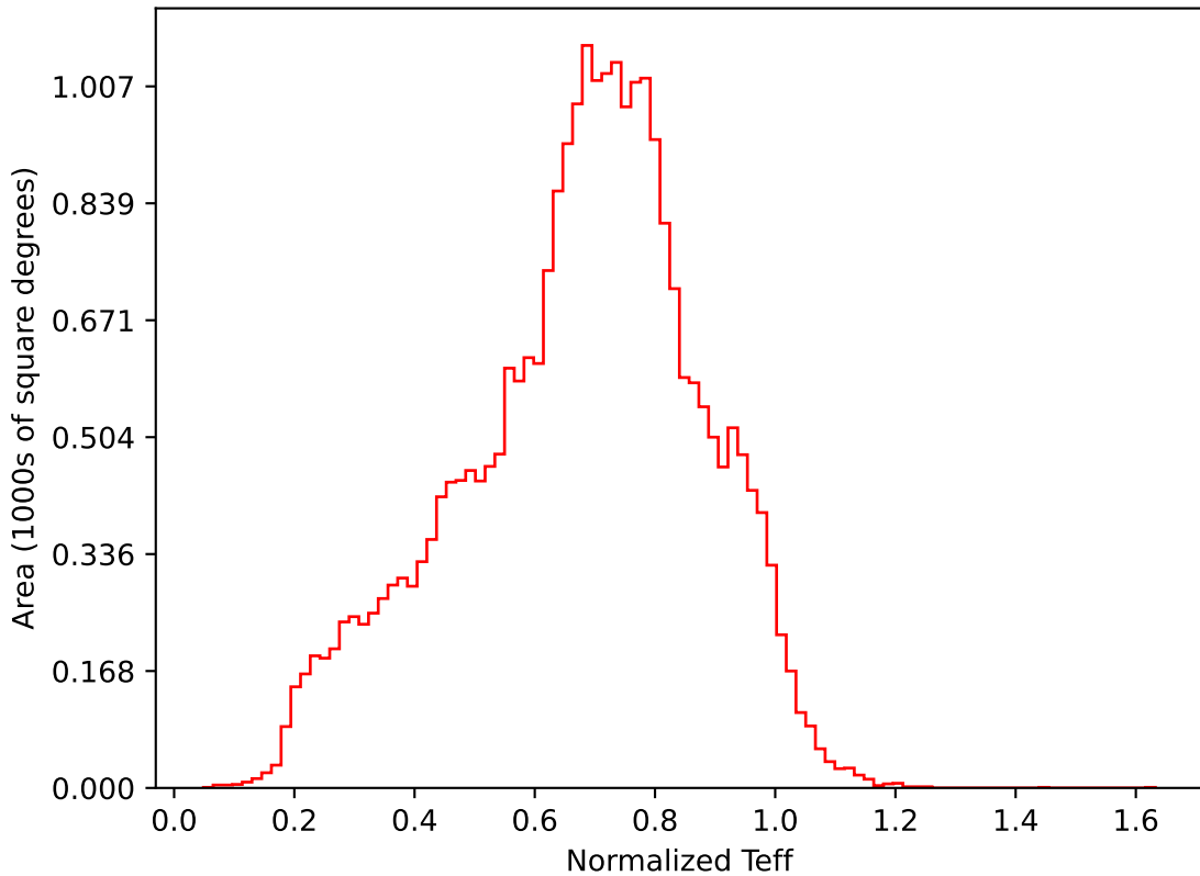
baseline_v3.3_10yrs All sky i band: Normalized Teff
