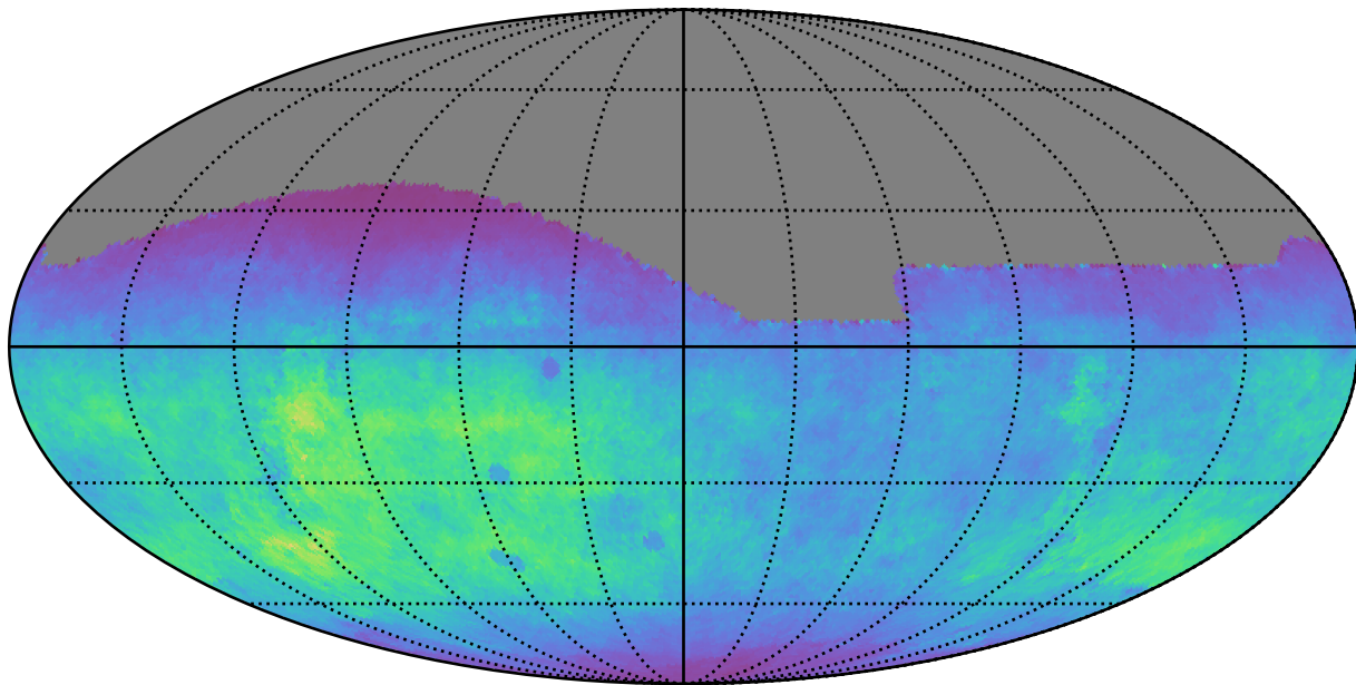
baseline_v3.3_10yrs All sky g band: Normalized Teff
