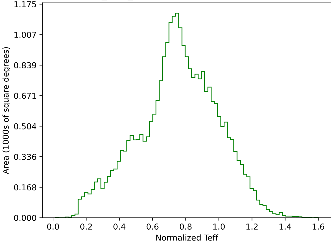
baseline_v3.3_10yrs All sky g band: Normalized Teff
