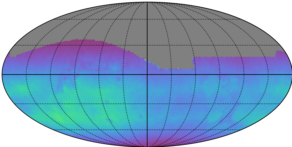
baseline_v3.3_10yrs All sky all bands: Normalized Teff
