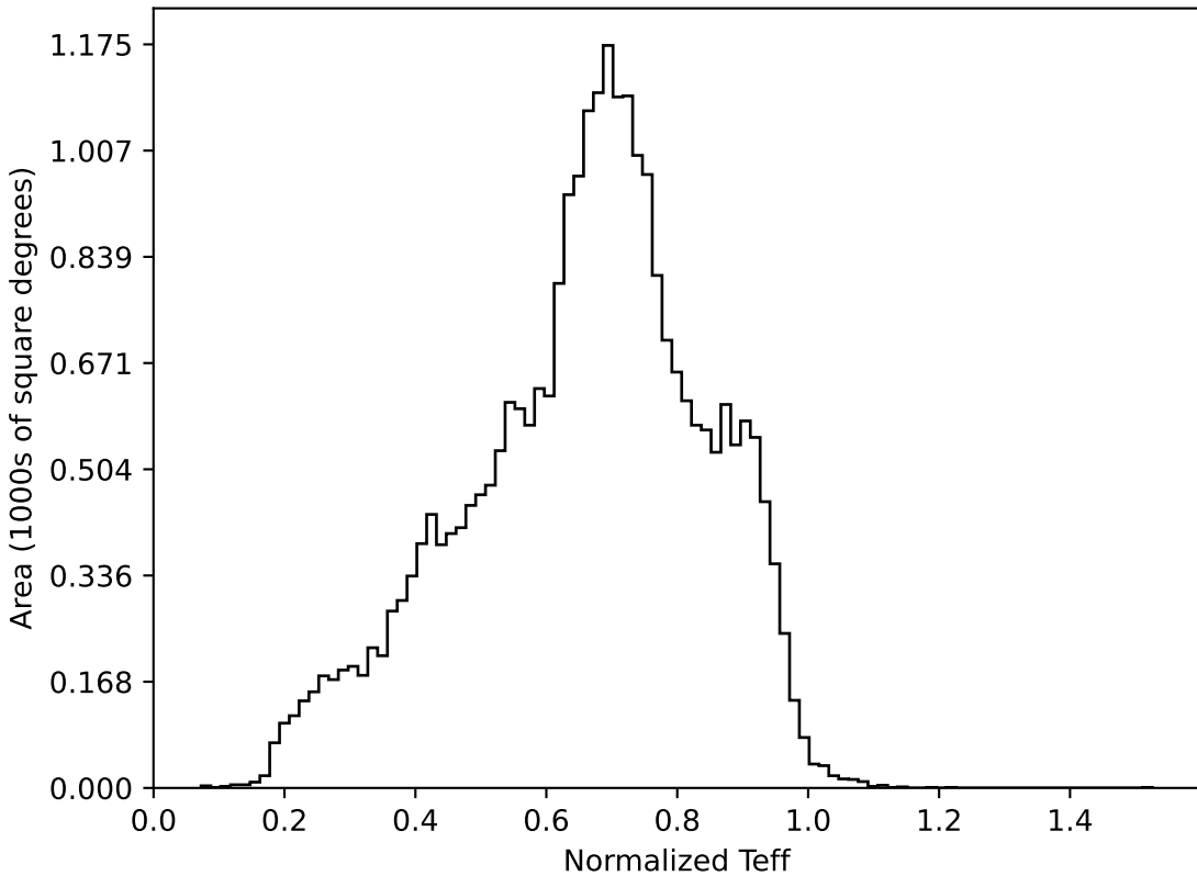
baseline_v3.3_10yrs All sky all bands: Normalized Teff
