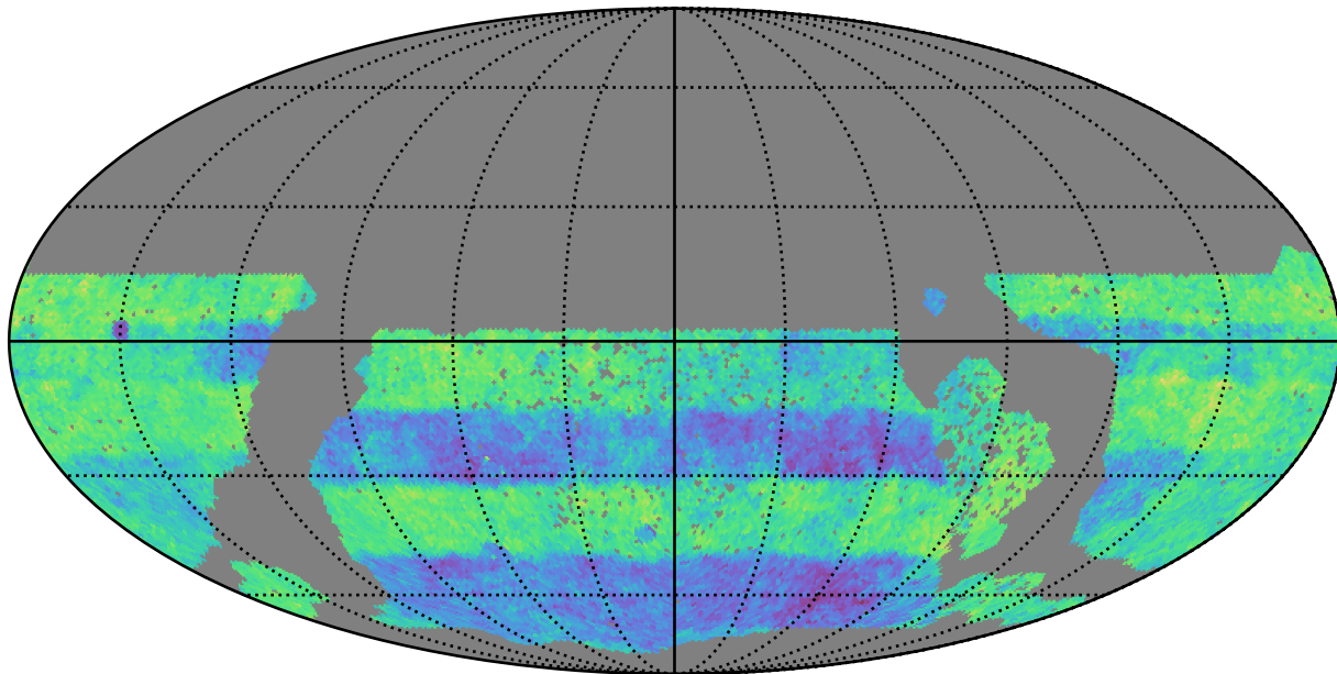
baseline_v3.3_10yrs WFD: Normalized Proper Motion Uncert @ 24.0
