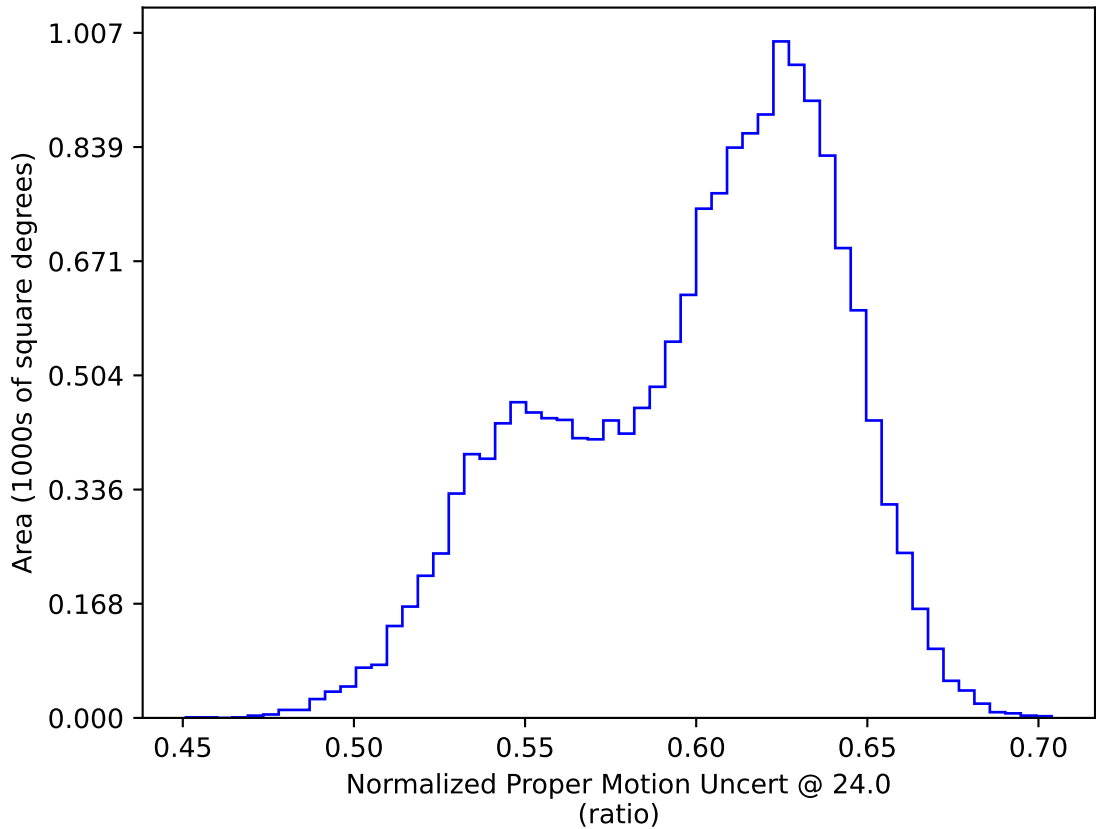
baseline_v3.3_10yrs WFD: Normalized Proper Motion Uncert @ 24.0
