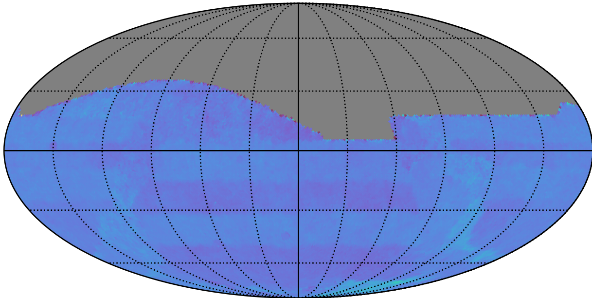
baseline_v3.3_10yrs All sky: Normalized Proper Motion Uncert @ 24.0
