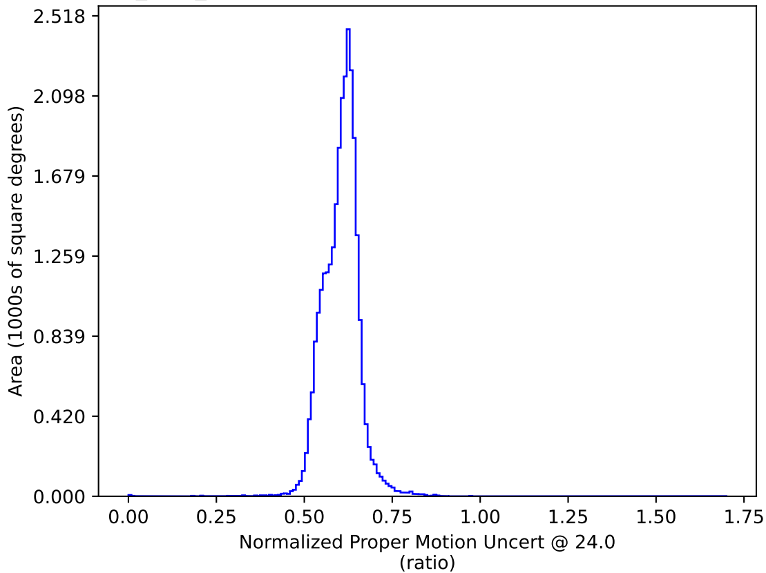
baseline_v3.3_10yrs All sky: Normalized Proper Motion Uncert @ 24.0
