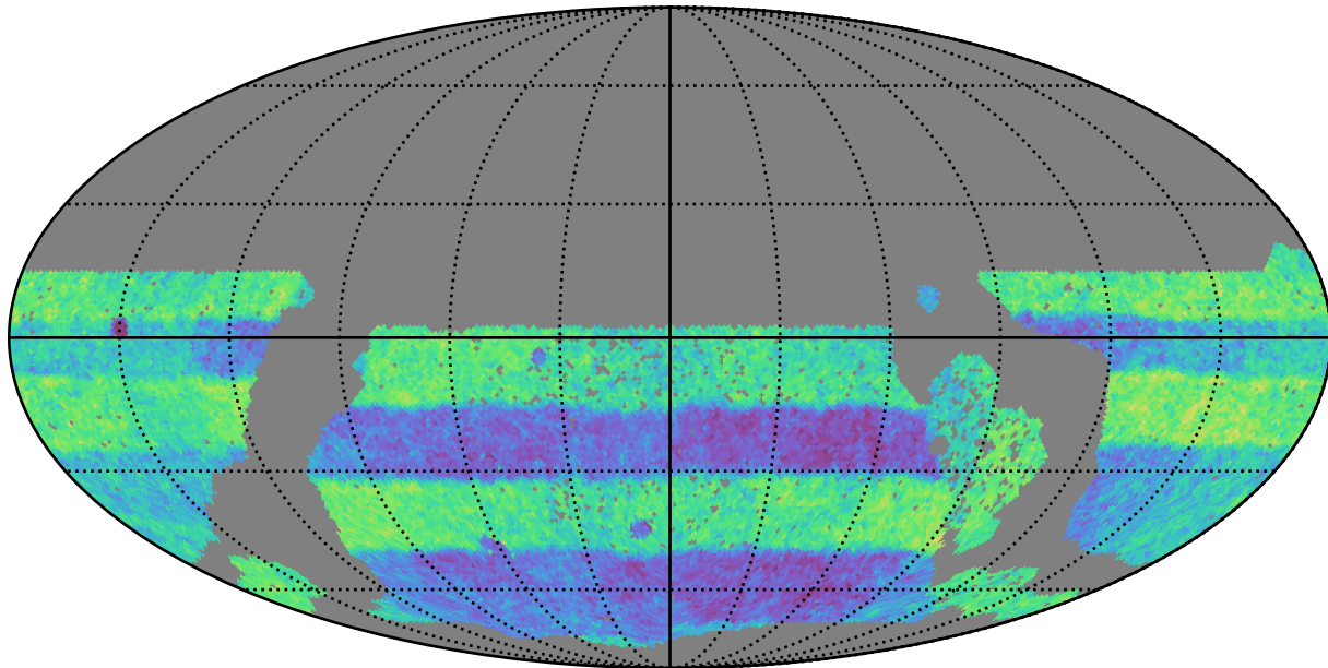
baseline_v3.3_10yrs WFD: Normalized Proper Motion Uncert @ 20.5
