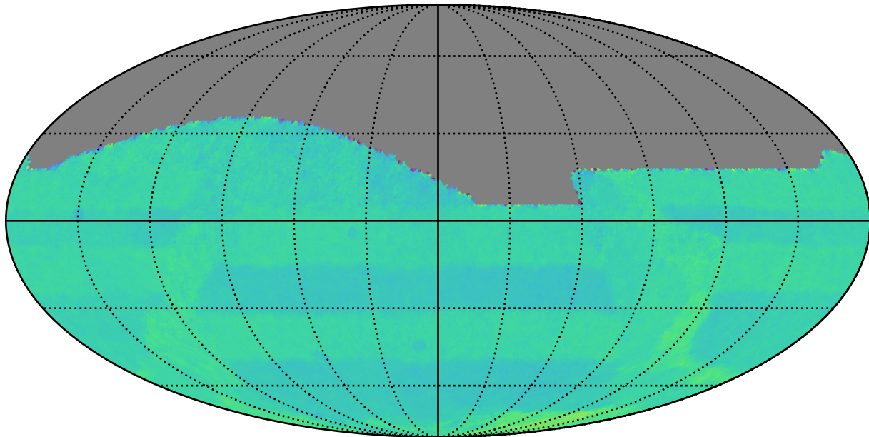
baseline_v3.3_10yrs All sky: Normalized Proper Motion Uncert @ 20.5
