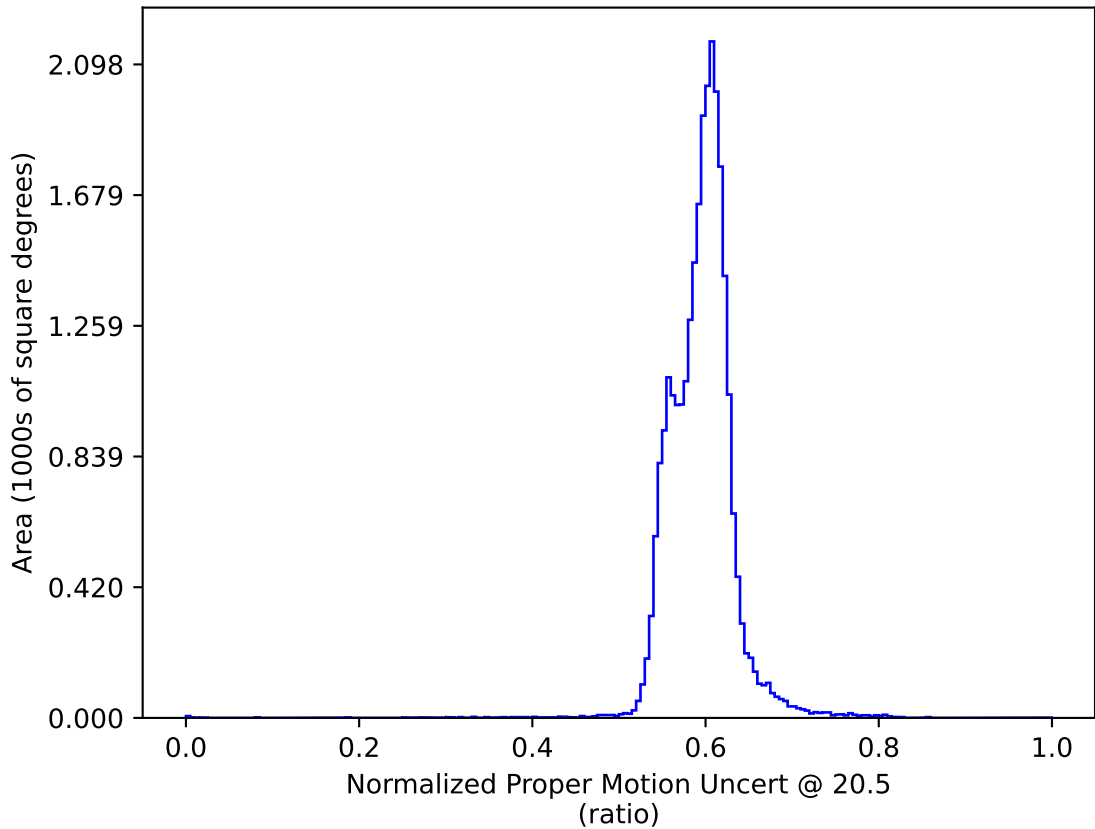
baseline_v3.3_10yrs All sky: Normalized Proper Motion Uncert @ 20.5
