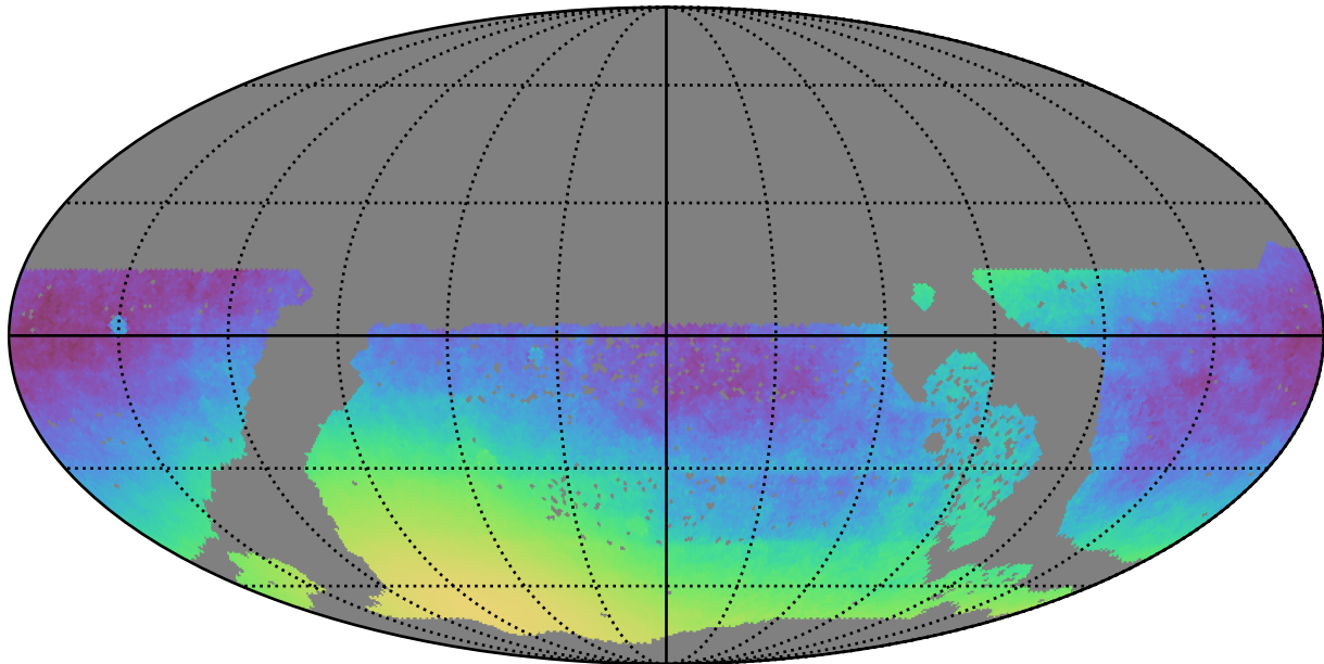
baseline_v3.3_10yrs WFD: Normalized Parallax Uncert @ 24.0
