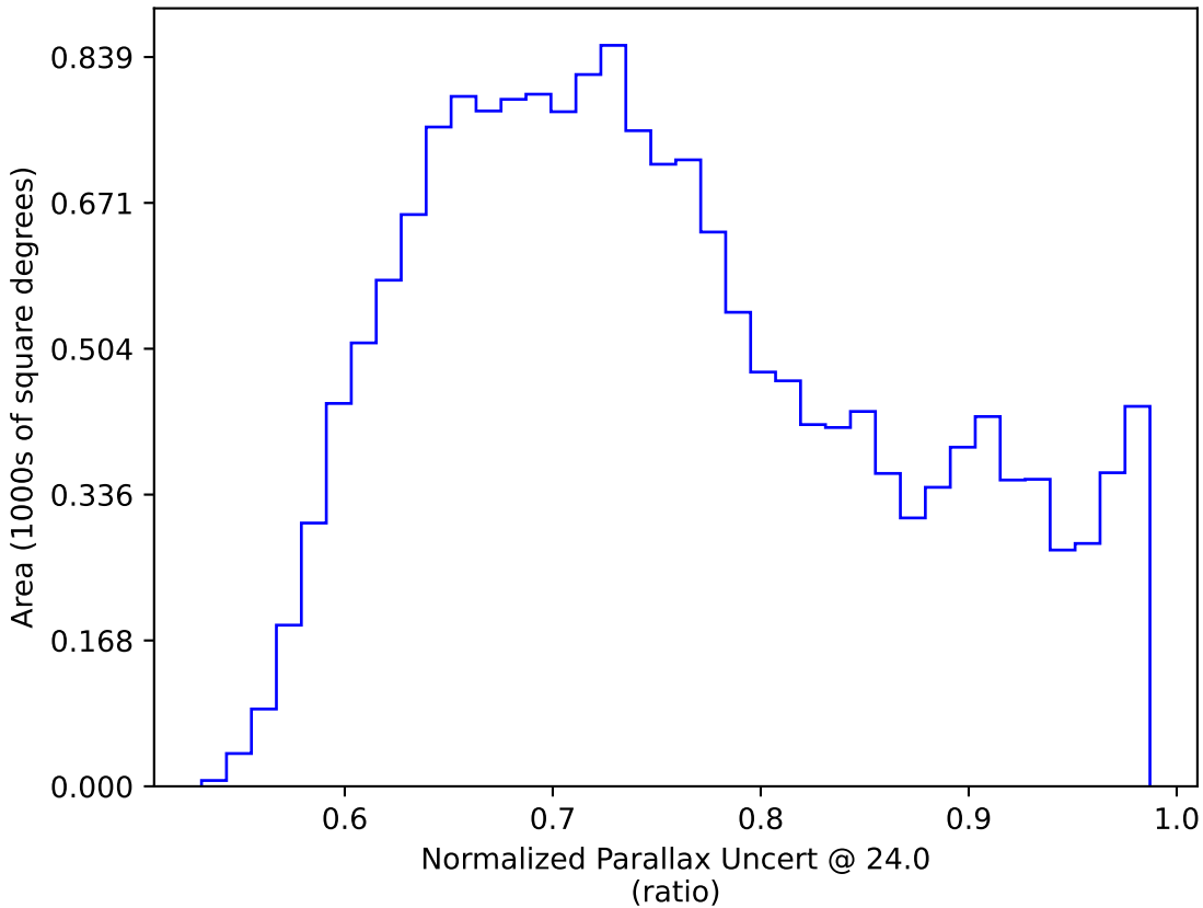
baseline_v3.3_10yrs WFD: Normalized Parallax Uncert @ 24.0
