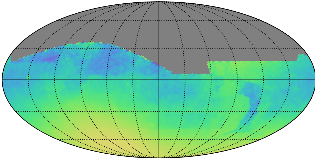
baseline_v3.3_10yrs All sky: Normalized Parallax Uncert @ 24.0
