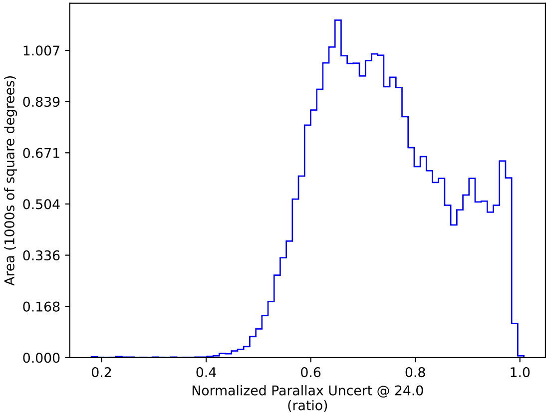
baseline_v3.3_10yrs All sky: Normalized Parallax Uncert @ 24.0
