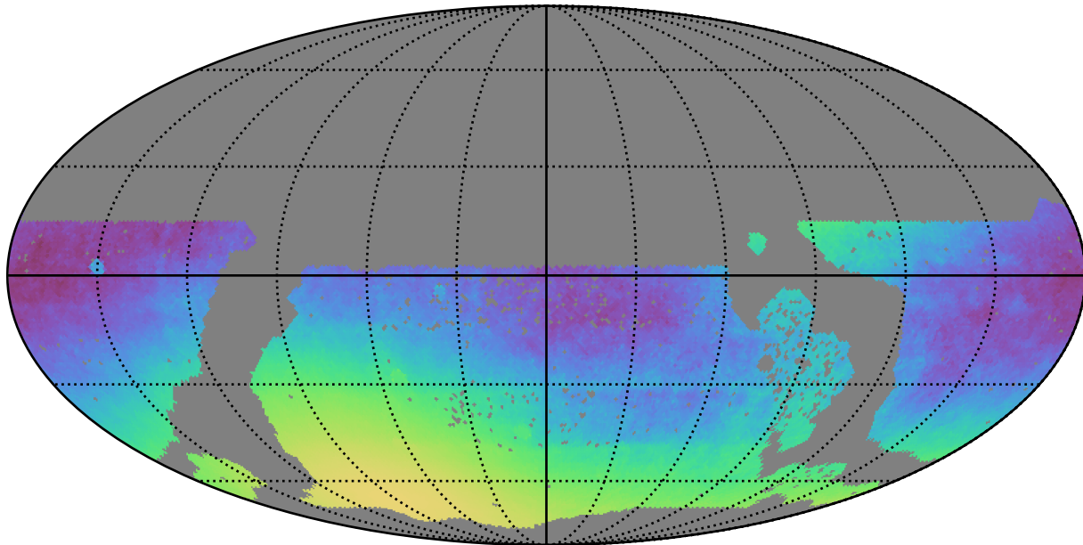
baseline_v3.3_10yrs WFD: Normalized Parallax Uncert @ 22.4
