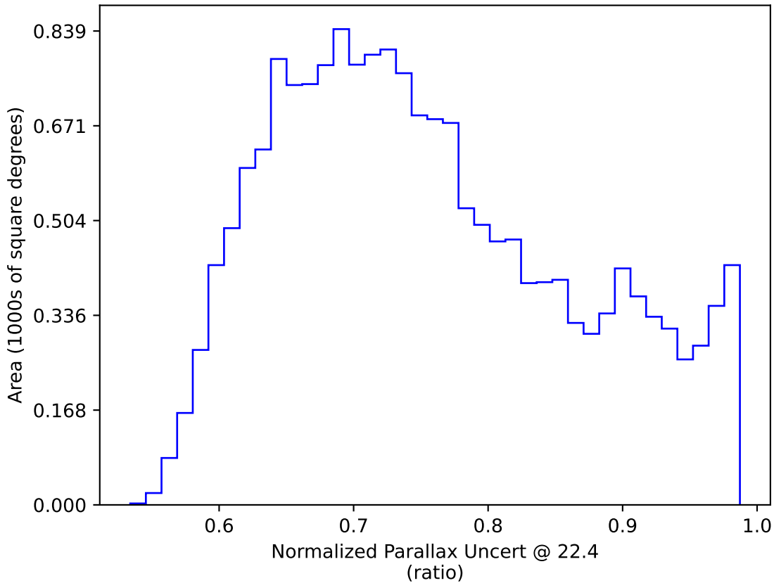
baseline_v3.3_10yrs WFD: Normalized Parallax Uncert @ 22.4
